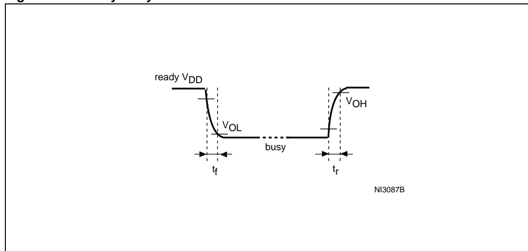
Figure 32. Ready/Busy AC waveform
