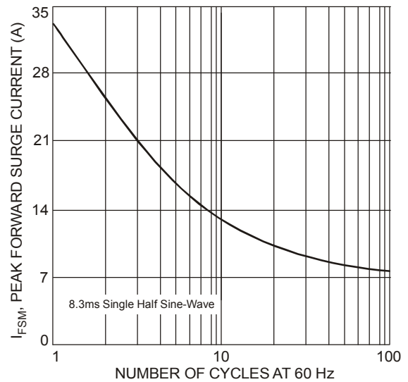
Figure 4 Maximum Non-Repetitive Peak Forward Surge Current
