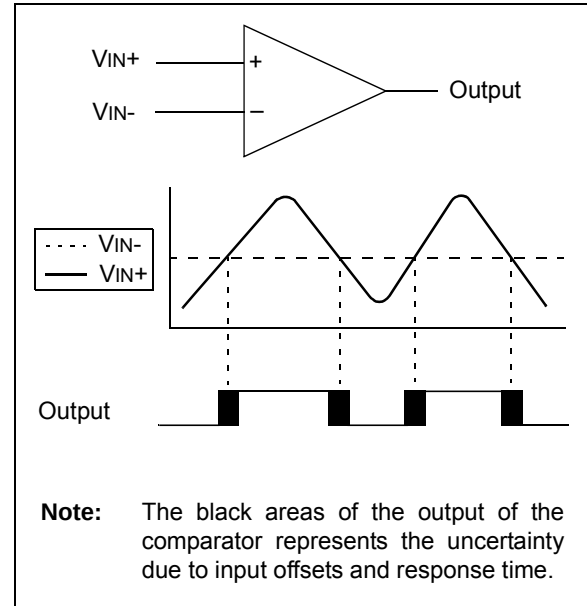
FIGURE 23-1: SINGLE COMPARATOR
