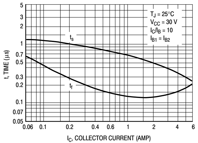
Figure 5. Turn-Off Time
