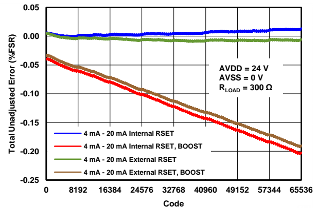
Figure 49. IOUT TUE vs CODE (4 mA to 20 mA)
