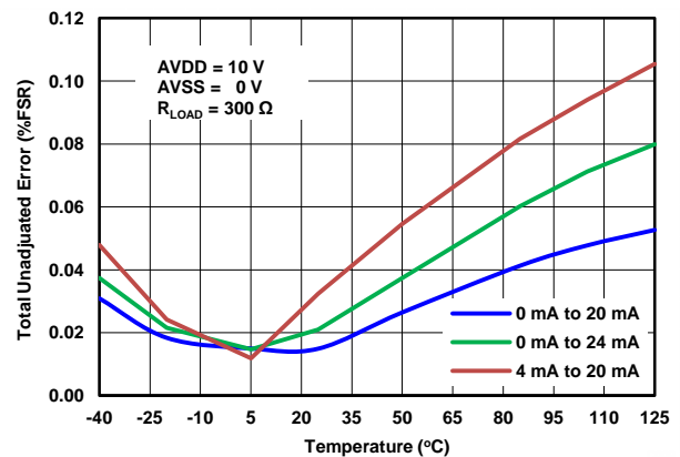
Figure 51. IOUT TUE vs TEMPERATURE (External R_{SET} )
