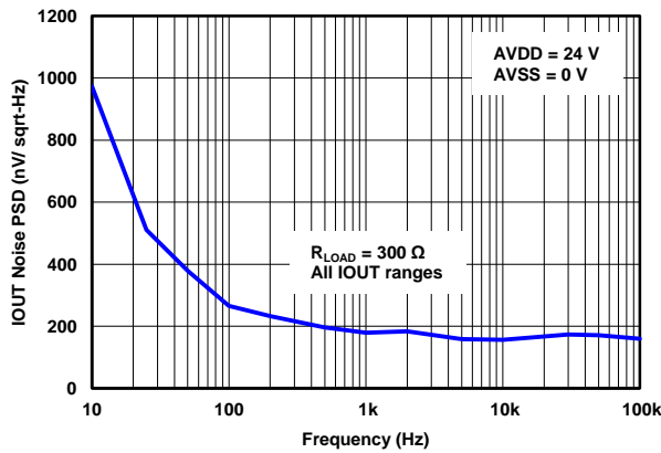
Figure 78. IOUT NOISE PSD vs FREQUENCY
