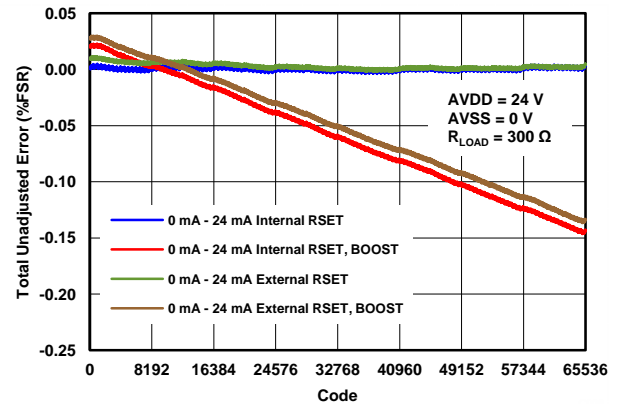
Figure 47. IOUT TUE vs CODE (0 mA to 24 mA)
