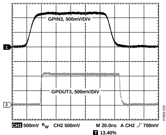
Figure 33. GPOUT3 Output vs. GPIN3 Input, V_{IN2} = 1.8V , V_{IN3} = 1.2V , 600\Omega Pull-Down, CH1 = GPIN3, CH2 = GPOUT3
