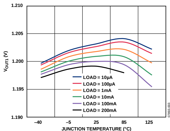
Figure 3. V_{OUT1} Output Voltage vs. Junction Temperature
