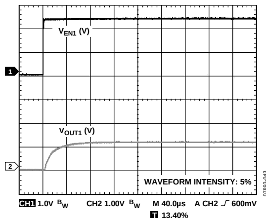
Figure 43. Typical Start-Up Time, V_{OUT1} = 1.2 V
