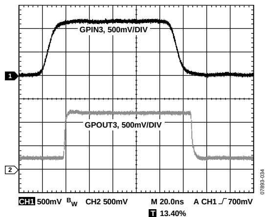
Figure 34. GPOUT3 Output vs. GPIN3 Input, V_{IN2} = 1.8V , V_{IN3} = 1.2V , 600\Omega Pull-Up, CH1 = GPIN3, CH2 = GPOUT3
