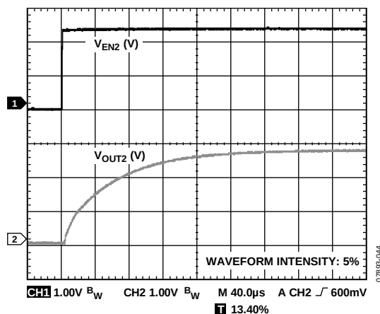
Figure 44. Typical Start-Up Time, V_{OUT2} = 2.8 V
