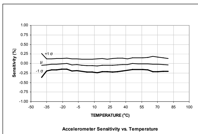
Figure 10. ADIS16350 Accelerometer Sensitivity vs. Temperature
