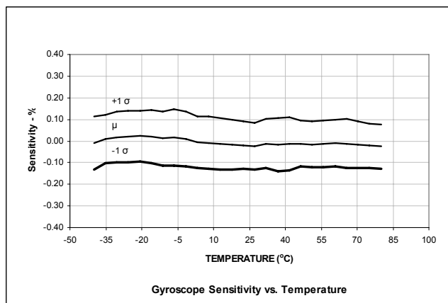
Figure 8. ADIS16355 Gyroscope Sensitivity vs. Temperature
