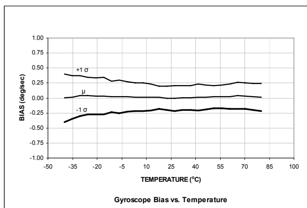
Figure 9. ADIS16350 Gyroscope Bias vs. Temperature
