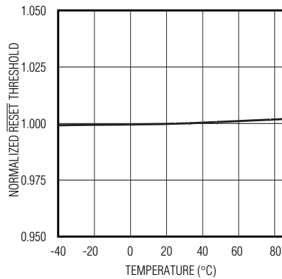
NORMALIZED \overline{RESET} THRESHOLD vs. TEMPERATURE
