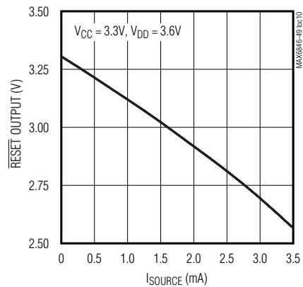
\overline{RESET} OUTPUT vs. SOURCE CURRENT
