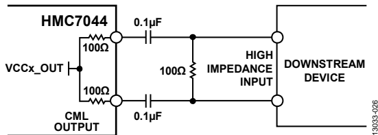
Figure 24. AC-Coupled CML (Internal) Output Driver
