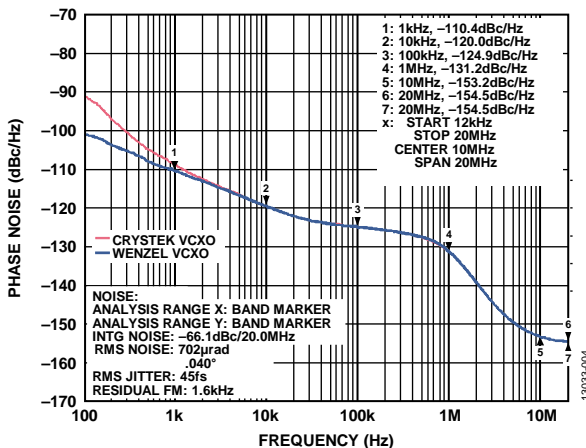
Figure 5. PLL2 Phase Noise vs. Frequency, VCXO Quality at 2457.6 MHz, Wide Loop Bandwidth
