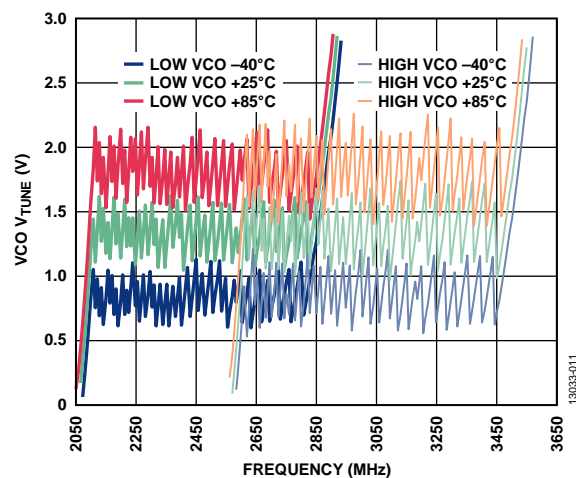
Figure 12. VCO V_{TUNE} vs. Frequency
