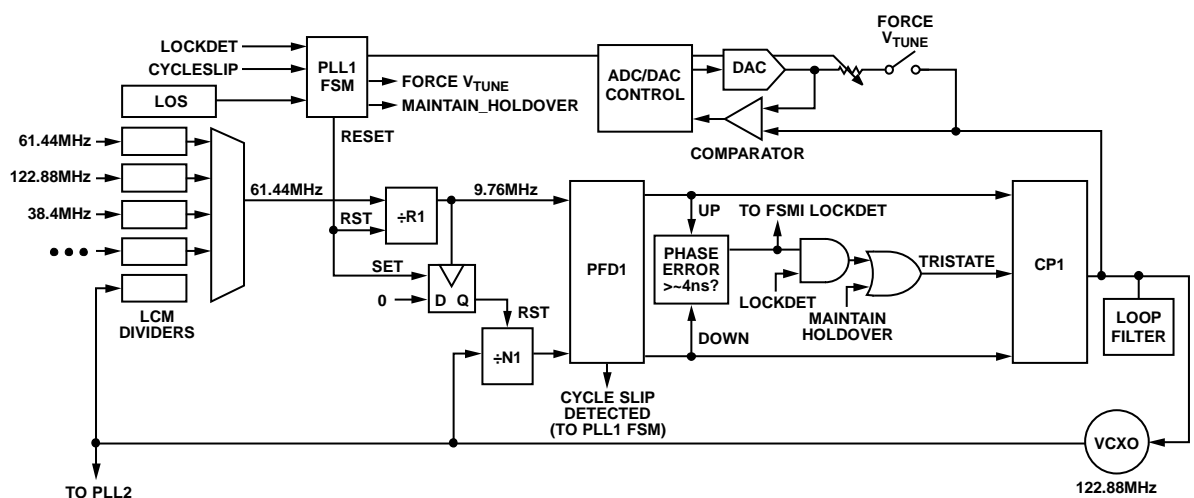
Figure 31. PLL1 Architecture with a Typical Frequency Configuration
