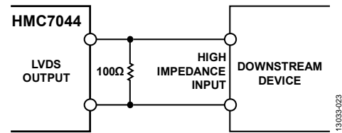
Figure 26. DC-Coupled LVDS Output Driver
