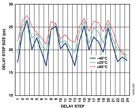
Figure 17. Analog Delay Step Size vs. Delay Step over Temperature, LVPECL at 1474.56 MHz
