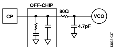
Figure 37. On-Chip RC Circuit
