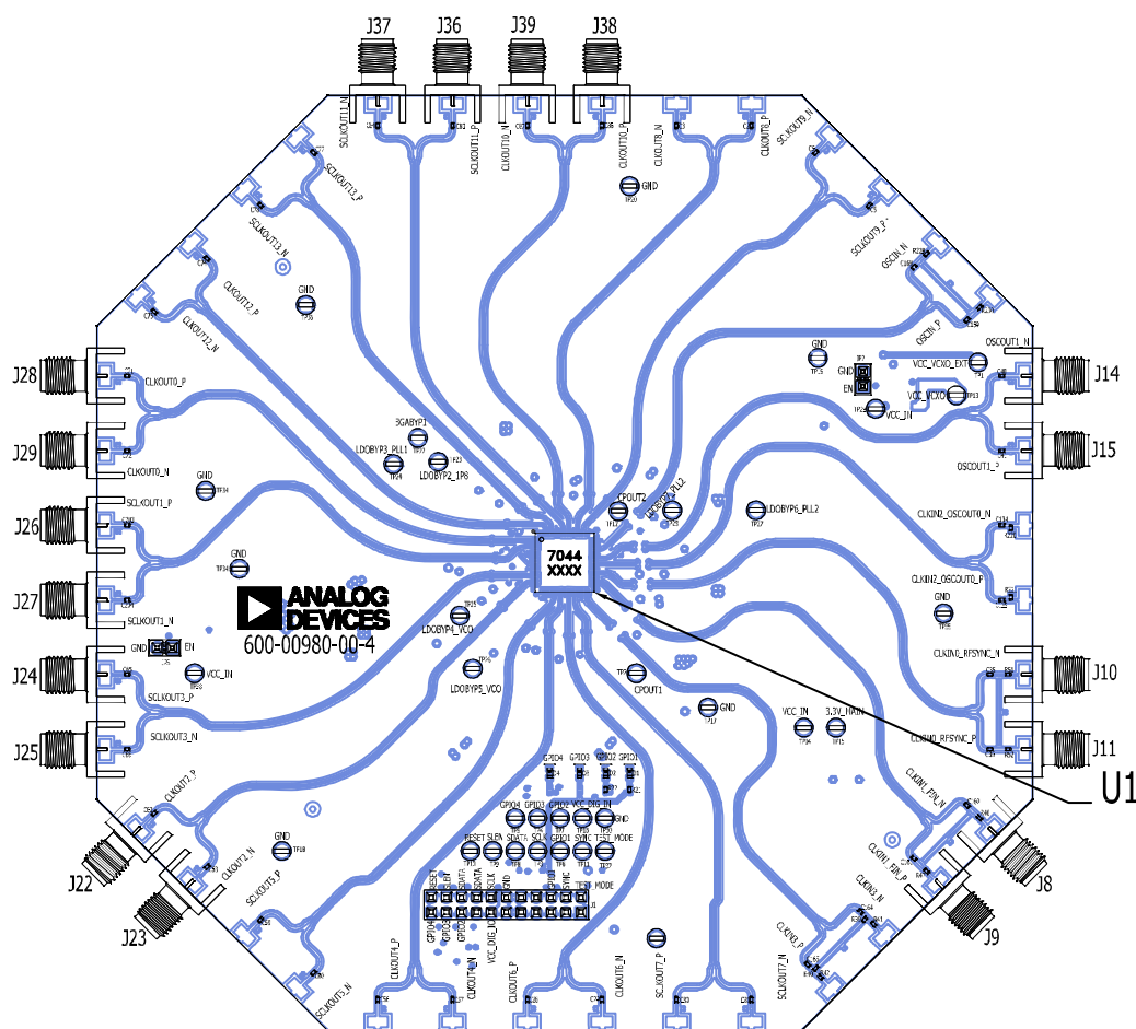
Figure 47. Evaluation PCB Layout, Top Side
