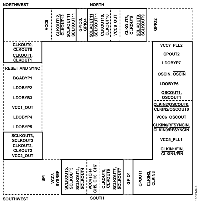
Figure 42. Clock Grouping
