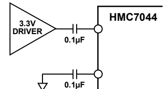
Figure 29. CLKIN0, CLKIN1, CLKIN2, CLKIN3, and OSCIN Input, Single-Ended Mode
