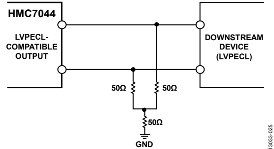
Figure 27. DC-Coupled LVPECL Output Driver
