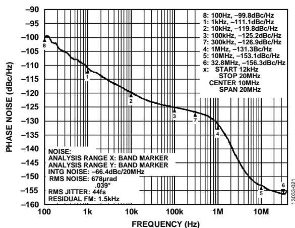
Figure 10. Phase Noise, CLKOUTx/CLKOUTx = 2457.6 MHz, Optimized for Best Integrated Jitter (12 kHz to 20 MHz)
