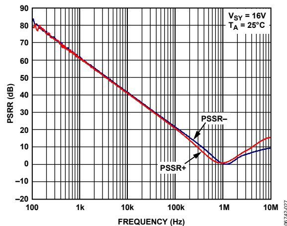
Figure 27. PSRR vs. Frequency, V_{SY} = 16 V
