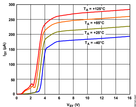
Figure 31. Supply Current vs. Supply Voltage AD8663
