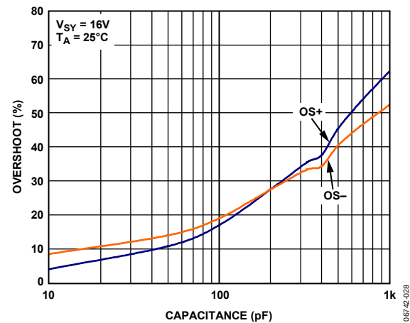
Figure 28. Small-Signal Overshoot vs. Load Capacitance, V_{SY} = 16 V
