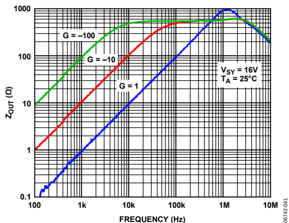
Figure 26. Closed-Loop Output Impedance vs. Frequency, V_{SY} = 16 V
