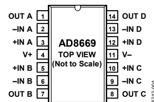
Figure 4. 14-Lead SOIC (R-14)
