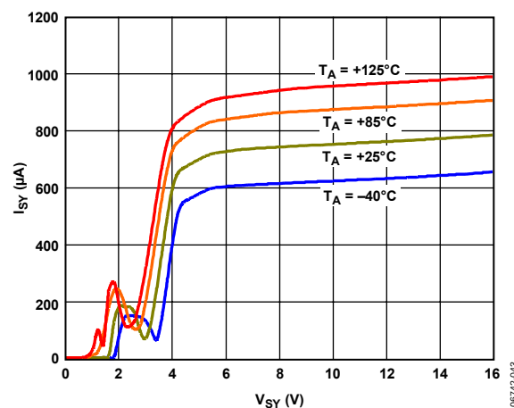
Figure 34. Supply Current vs. Supply Voltage AD8669
