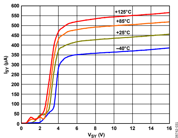
Figure 35. Supply Current vs. Supply Voltage AD8667
