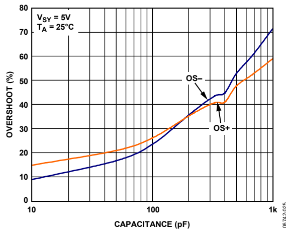
Figure 25. Small-Signal Overshoot vs. Load Capacitance, V_{SY} = 5 V
