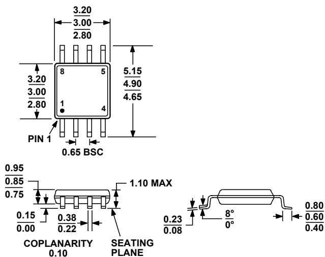
Figure 45. 8-Lead Mini Small Outline Package [MSOP] (RM-8)
