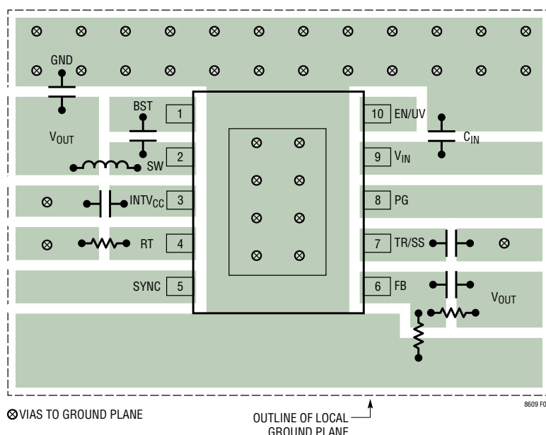
Figure 4. PCB Layout
