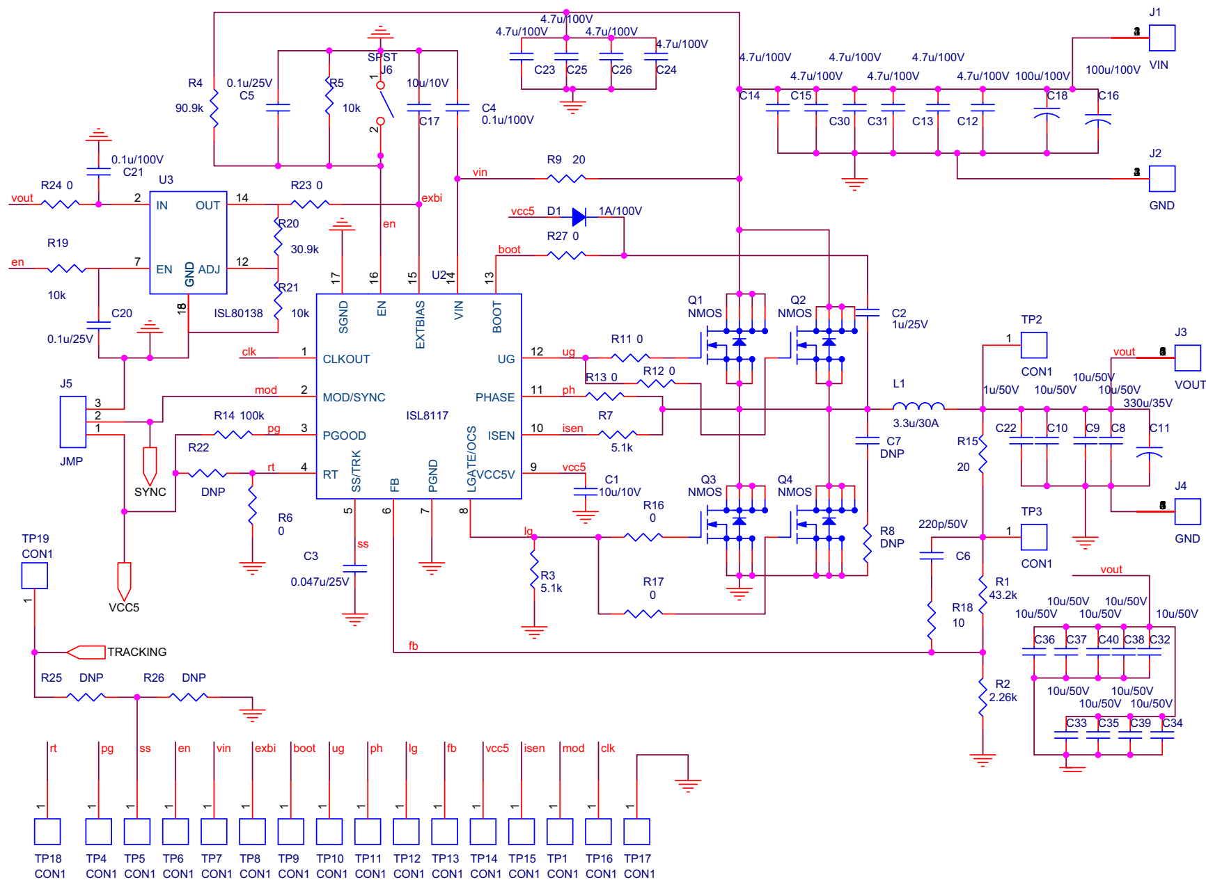
FIGURE 20. ISL8117EVAL2Z SCHEMATIC
