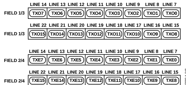
Figure 49. Teletext Control Registers
