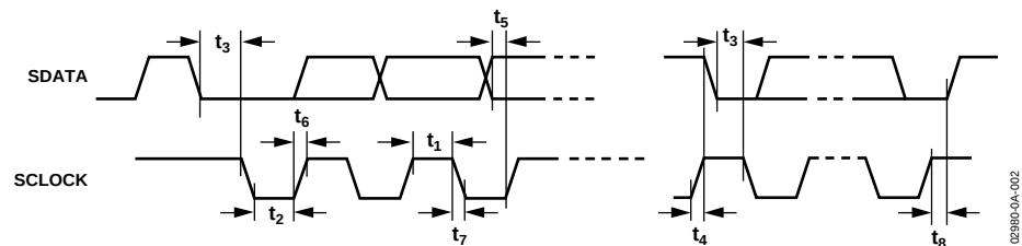
Figure 2. MPU Port Timing Diagram
