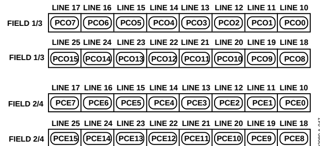
Figure 48. Pedestal Control Registers
