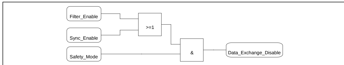
Figure 4.10 Flowchart – Data_Exchange_Disable
