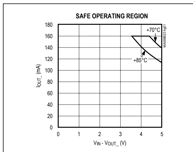
Figure 1. MAX8882/MAX8883 Safe Operating Region
