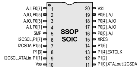
Figure 4. CY8C27243 20-Pin PSoC Device
