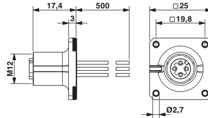
Dimensioned drawing
