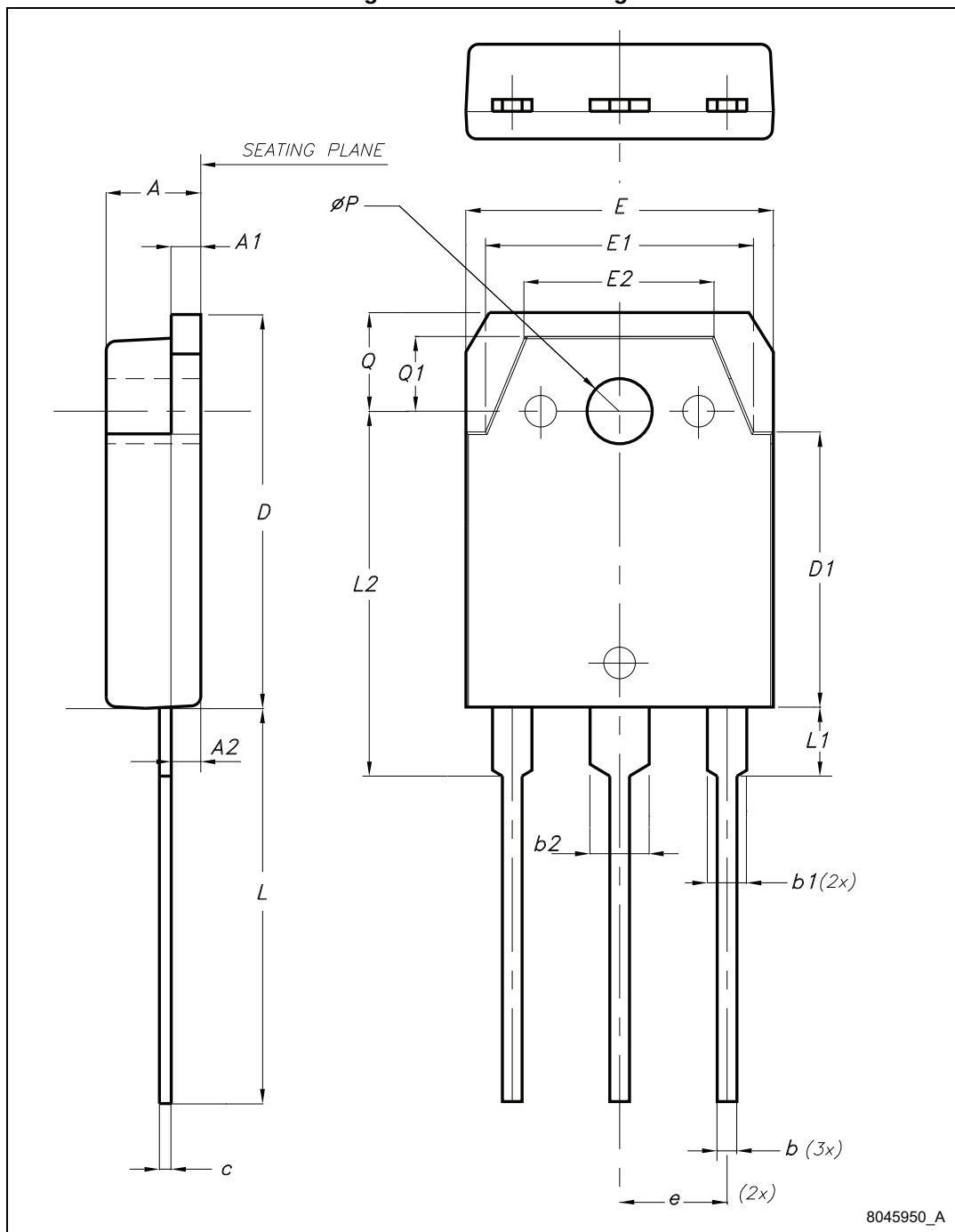
Figure 32. TO-3P drawing
