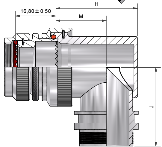
90° BACKSHELL - TYPE 2
