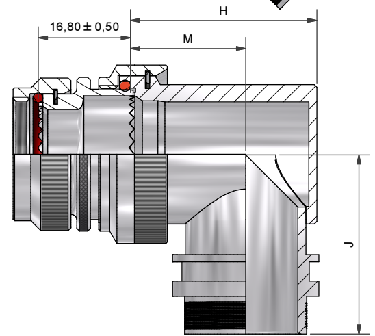
90° BACKSHELL - TYPE 2
