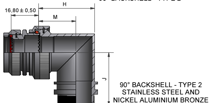
90° BACKSHELL - TYPE 2
