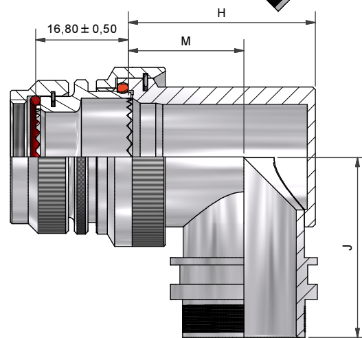
90° BACKSHELL - TYPE 2
