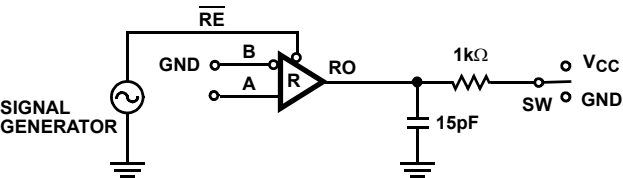
FIGURE 5. RECEIVER PROPAGATION DELAY AND DATA RATE
