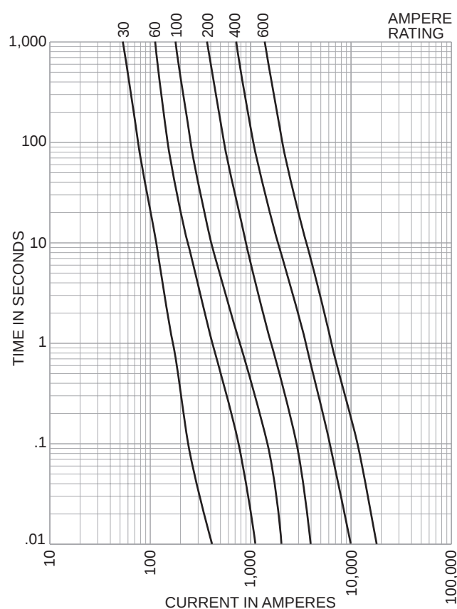
Time/Current-Curves
