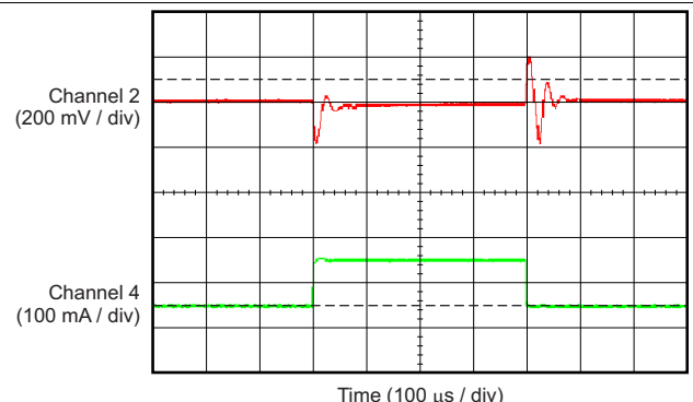
Figure 16. TPS70612 Load Transient (1 mA to 150 mA)
