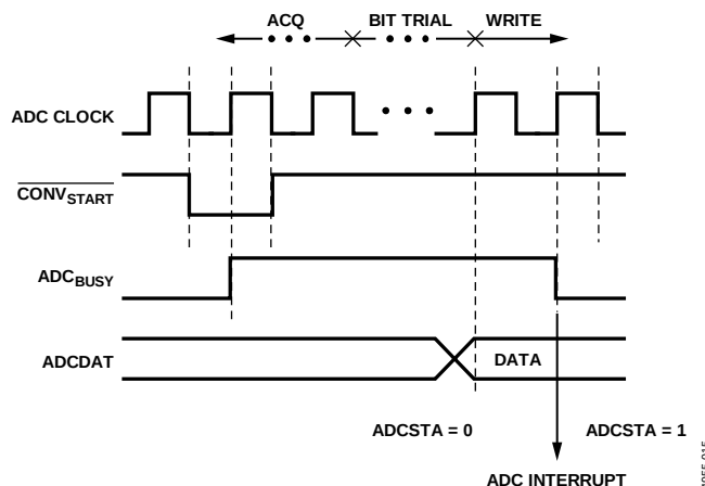
Figure 42. ADC Timing
