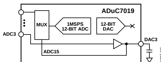
Figure 43. ADC3 Buffered Input
