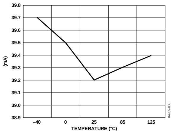
Figure 29. Current Consumption vs. Temperature @ CD = 0
