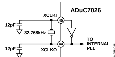
Figure 80. External Parallel Resonant Crystal Connections
