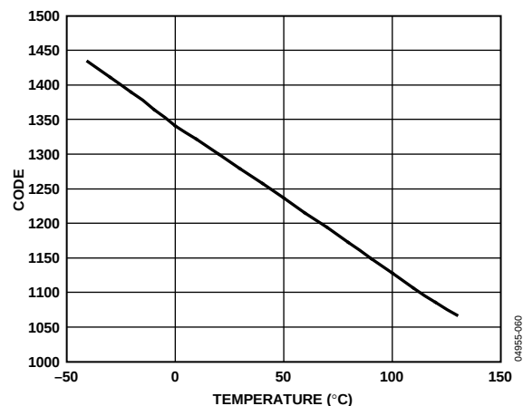
Figure 28. On-Chip Temperature Sensor Voltage Output vs. Temperature
