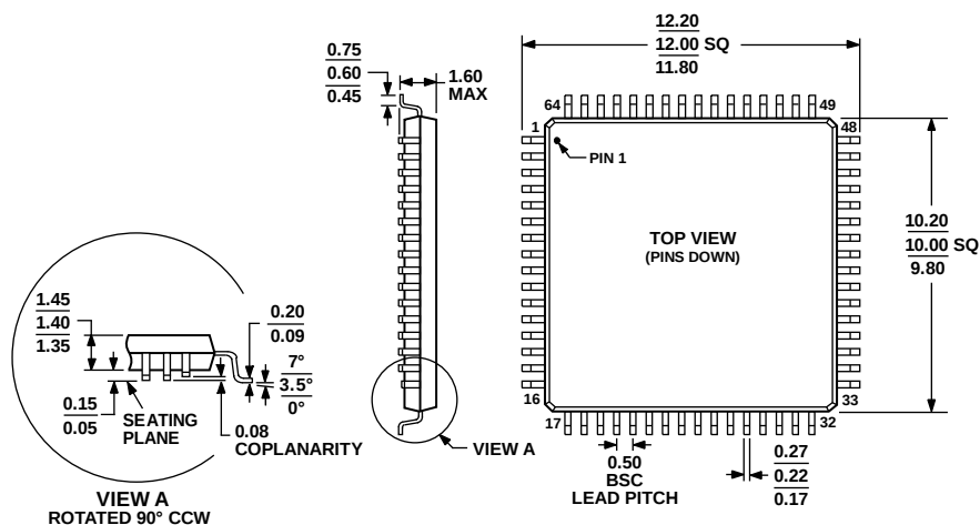
Figure 86. 64-Lead Low Profile Quad Flat Package [LQFP] (ST-64-2)
