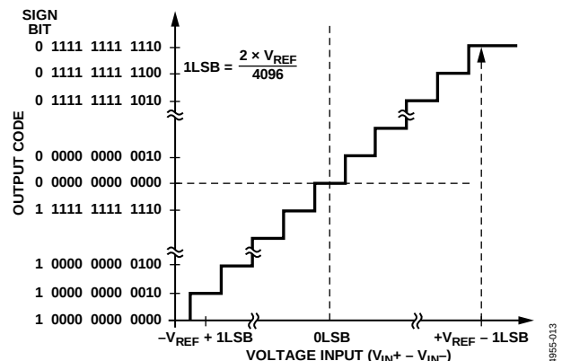
Figure 40. ADC Transfer Function in Differential Mode
