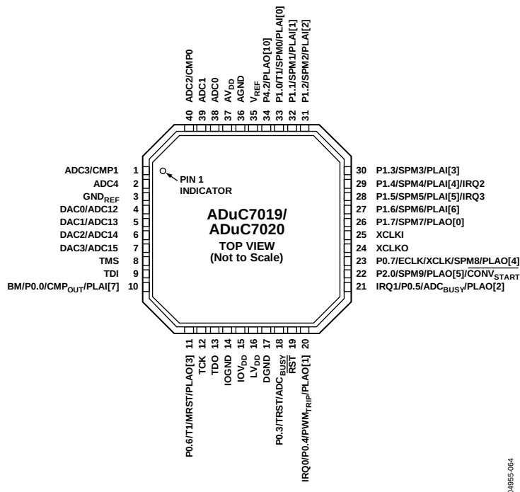
Figure 10. 40-Lead LFCSP_VQ Pin Configuration (ADuC7019/ADuC7020)
