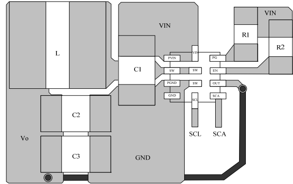
Figure 4: Recommended Layout
