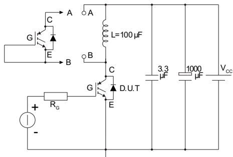
Figure 28. Test circuit for inductive load switching
