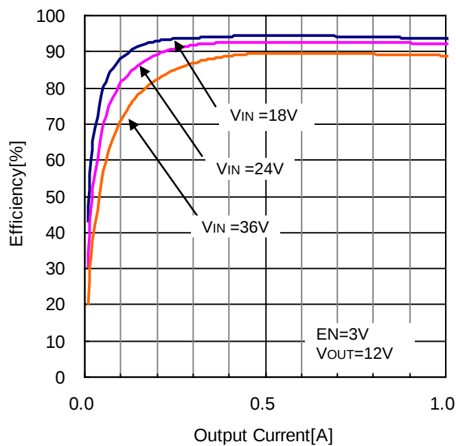
Figure 20. Efficiency vs Output Current ( V_{OUT} = 12V , L = 6.8\mu H )
