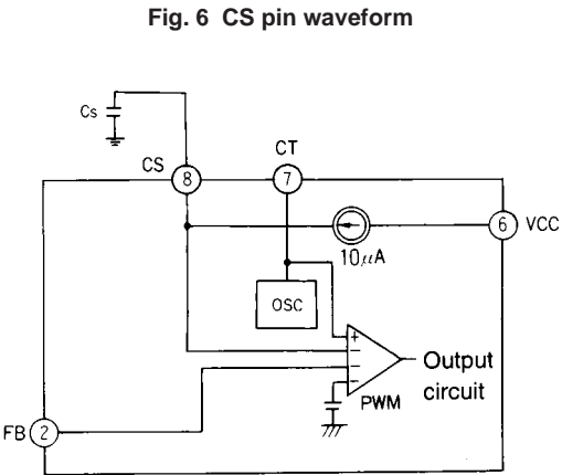
Fig. 7 Soft-start circuit
