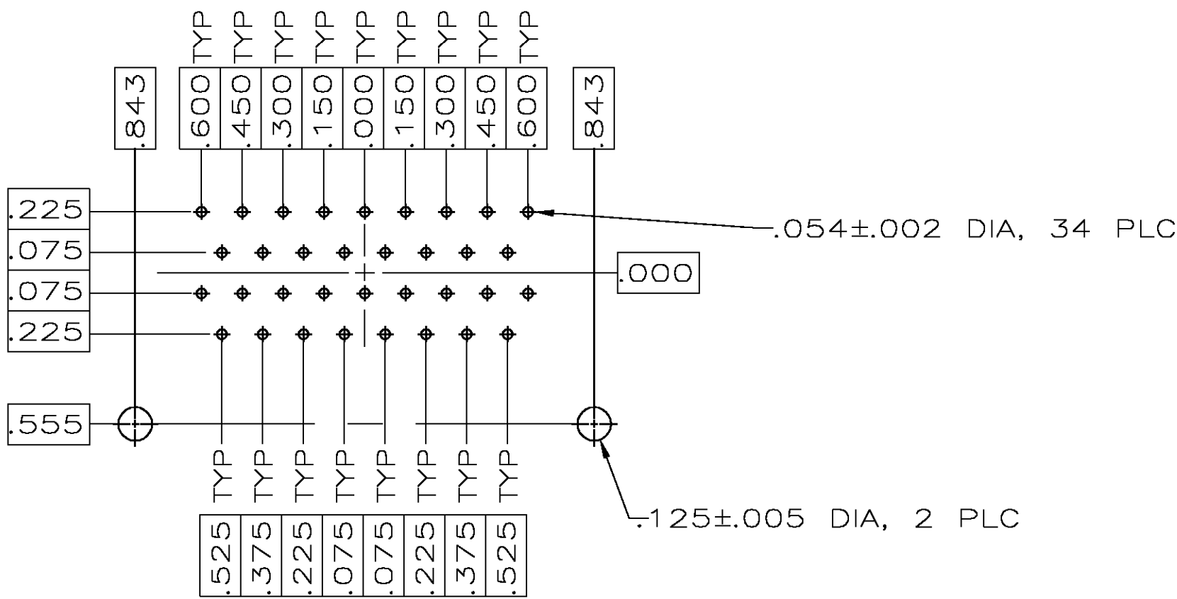
RECOMMENDED P.C. BOARD LAYOUT
