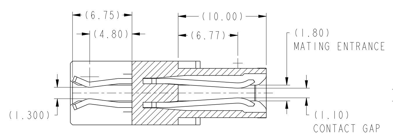
SECTION C-C
