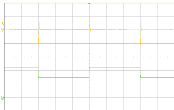
Figure 4 Dynamic response for 25% load step (50% ~ 75% ~ 50%) and 0.1A/µs slew rate, (2ms/div), see Figure 11 for test configuration; CH1-output voltage (50mV/div); CH2-output current (10A/div)
