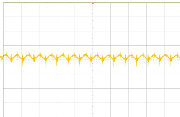
Figure 3 Input reflected ripple current (5µs/div, 5mA/div), see Figure 16 for test configuration
