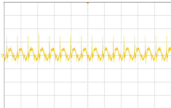
Figure 2 Output ripple & noise (5µs/div, 20mV/div), see Figure 16 for test configuration
