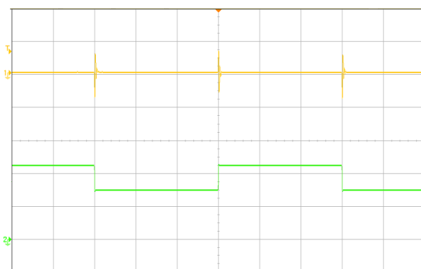
Figure 5 Dynamic response for 25% load step (50% ~ 75% ~ 50%) and 1A/µs slew rate, (2ms/div), see Figure 11 for test configuration; CH1-output voltage (200mV/div); CH2-output current (10A/div)
