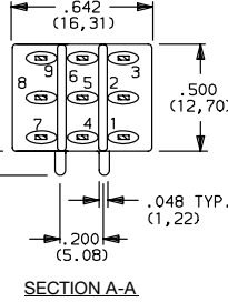
E301MD1AV2BE Vertical Actuation 3PDT
