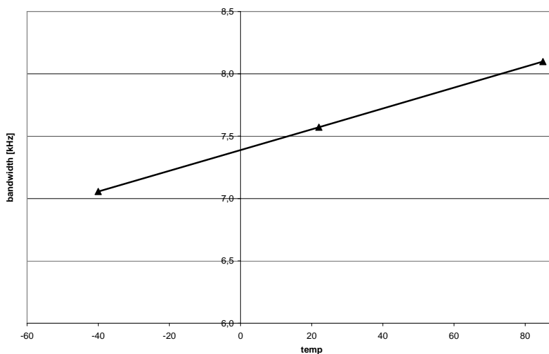
Figure 8 Typical temperature dependency of bandwidth BW
