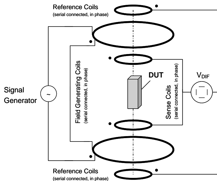
Figure 12. Helmholtz setup for electrical characteristics
