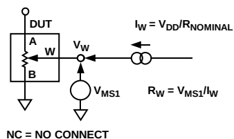
Figure 33. Wiper Resistance
