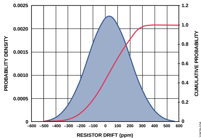
Figure 26. Resistor Lifetime Drift
