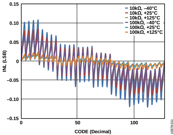
Figure 11. INL vs. Code (AD5123)
