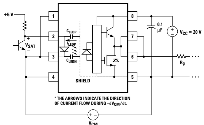
A high CMR LED drive circuit must keep the LED on during common mode transients. This is achieved by over-driving the LED current beyond the input threshold so that it is not pulled below the threshold during a transient. A minimum LED current of 10 mA provides adequate margin over the maximum I_{FLH} of 8 mA to achieve 10 kV/ \mu s CMR.
