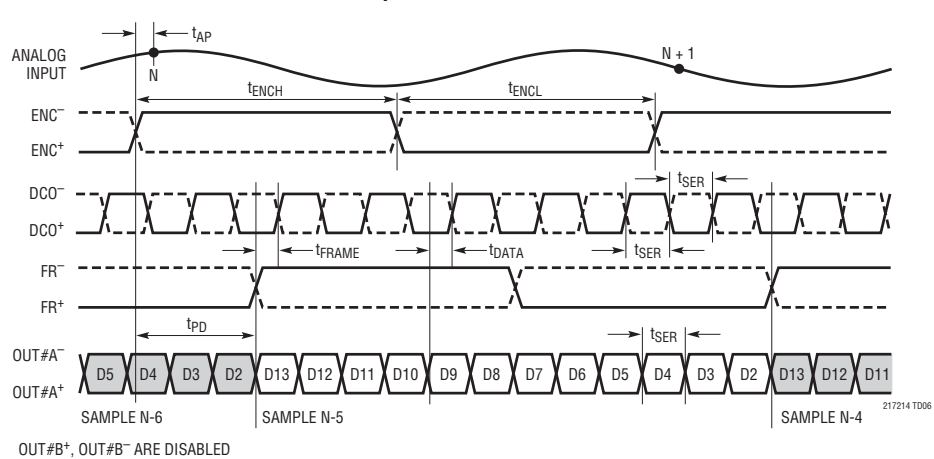
1-Lane Output Mode, 12-Bit Serialization
