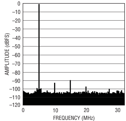
LTC2172-14: 8k Point FFT, f_{IN} = 5\text{MHz} -1dBFS, 65Msps
