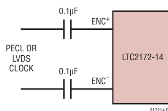
Figure 13. PECL or LVDS Encode Drive
