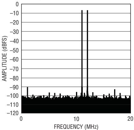
LTC2171-14: 8k Point 2-Tone FFT, f_{IN} = 68\text{MHz}, 69\text{MHz} , -1dBFS, 40Msps
