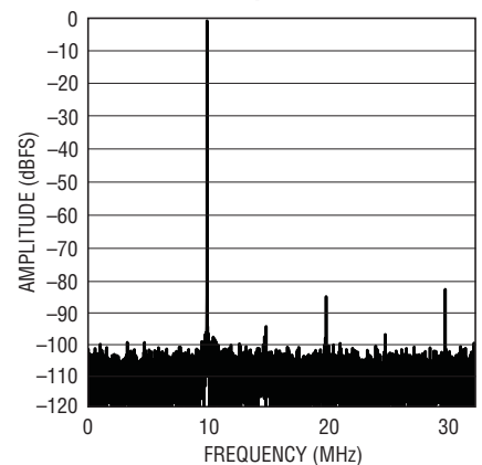
LTC2172-14: 8k Point FFT, f_{IN} = 140\text{MHz} -1dBFS, 65Msps
