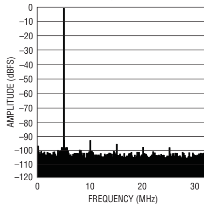
LTC2172-14: 8k Point FFT, f_{IN} = 70\text{MHz} -1dBFS, 65Msps
