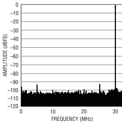
LTC2172-14: 8k Point FFT, f_{IN} = 30\text{MHz} -1dBFS, 65Msps
