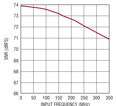
LTC2172-14: SNR vs Input Frequency, -1dBFS, 2V Range, 65Msps
