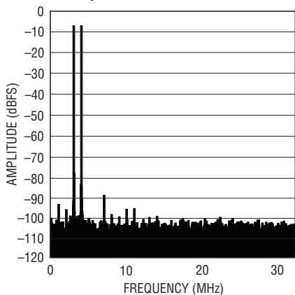
LTC2172-14: 8k Point 2-Tone FFT, f_{IN} = 68\text{MHz}, 69\text{MHz} , -1dBFS, 65Msps
