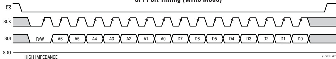
SPI Port Timing (Write Mode)
