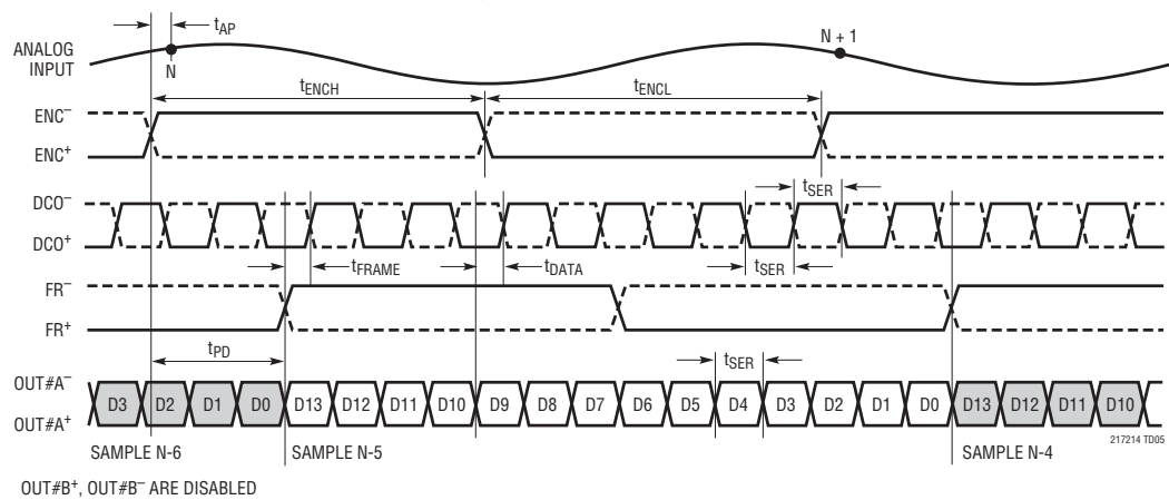
1-Lane Output Mode, 14-Bit Serialization
