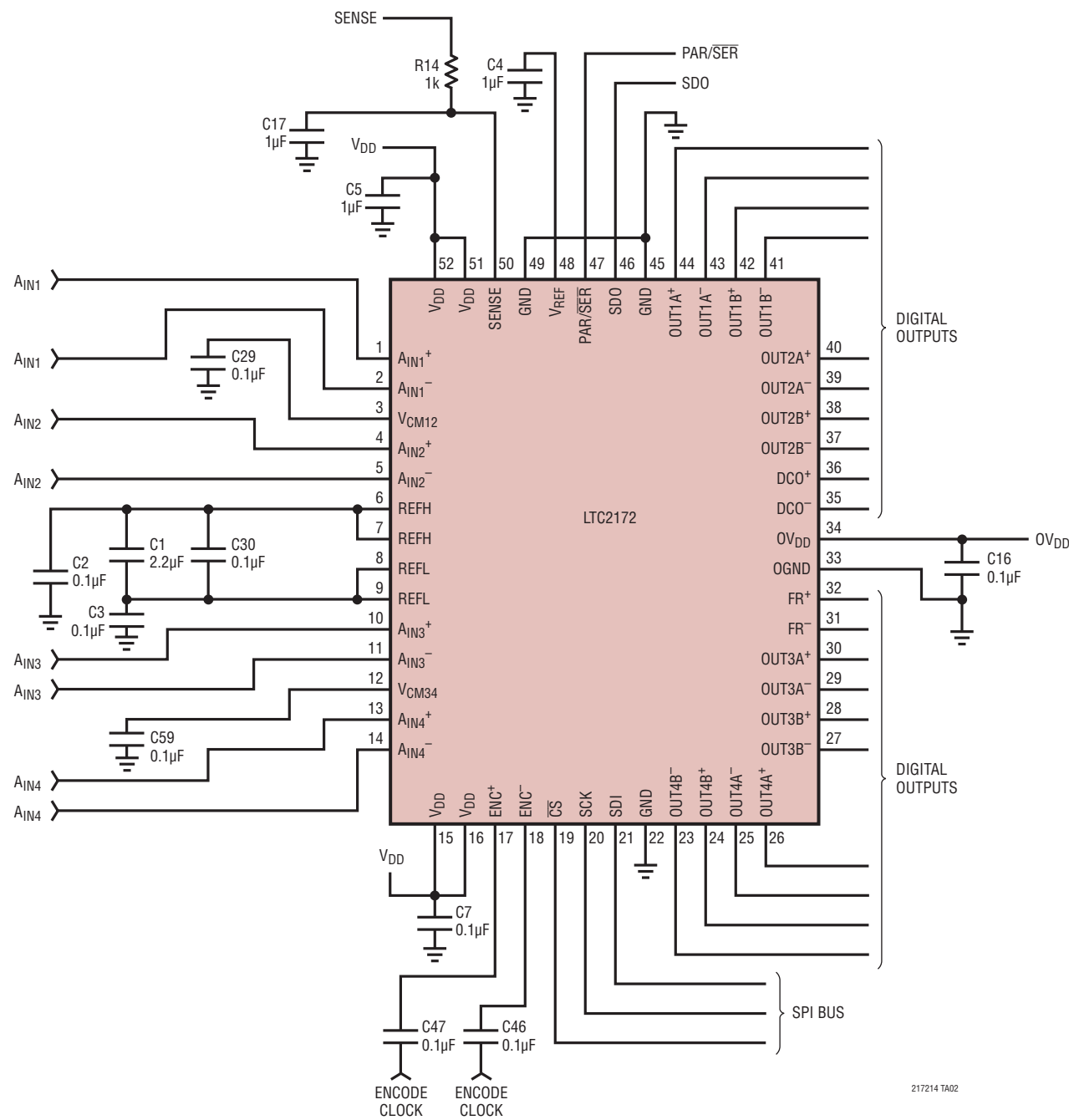
LTC2172 Schematic
