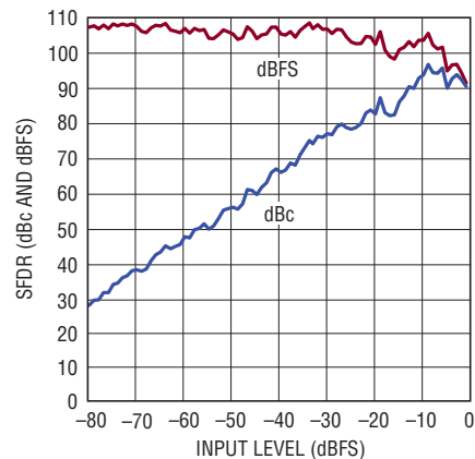
LTC2171-14: SFDR vs Input Level, f_{IN} = 70\text{MHz} , 2V Range, 40Msps
