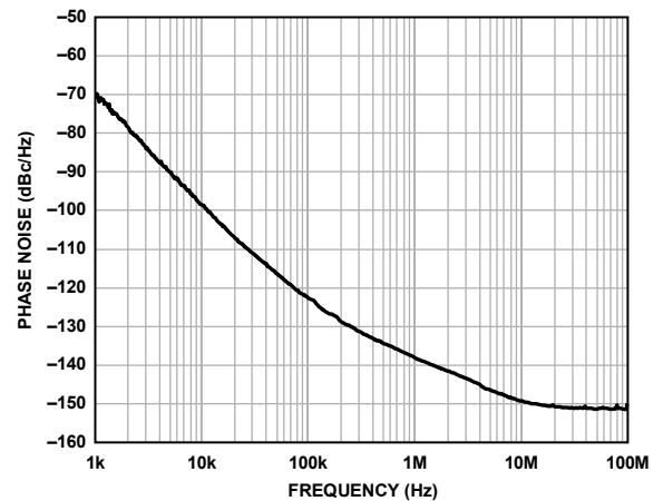
Figure 23. Internal VCO Phase Noise (Absolute), LVDS Output @ 573 MHz
