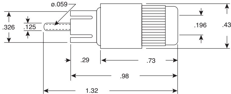
Dimensions: In.
