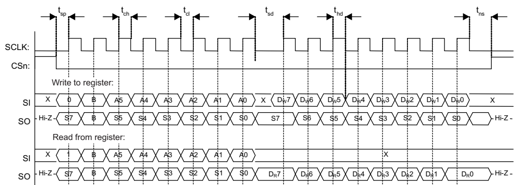
Figure 5-3. Configuration Registers Write and Read Operations
