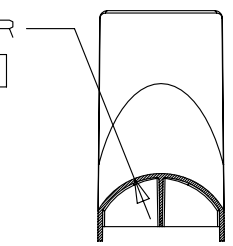
SECTION A-A (BEND RADIUS CONTROL)
