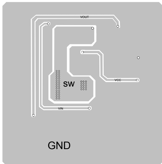
Figure 13— Sample Board Layout
