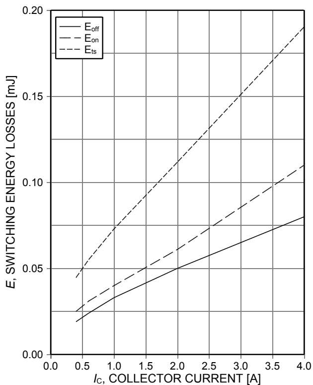
Figure 13. Typical switching energy losses as a function of collector current (inductive load, T_{vj}=175^\circ\text{C} , V_{CE}=400\text{V} , V_{GE}=15/0\text{V} , r_G=43\Omega , Dynamic test circuit in Figure E)
