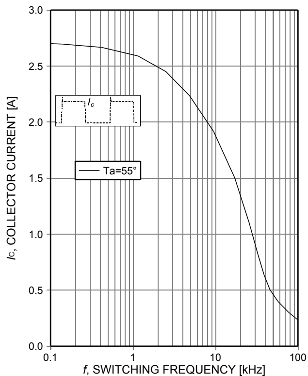
Figure 1. Collector current as a function of switching frequency ( T_{vj} \leq 175^\circ\text{C} , T_a=55^\circ\text{C} , D=0.5 , V_{CE}=400\text{V} , V_{GE}=15/0\text{V} , r_G=43\Omega , PCB mounting, 6cm 2 Cu, P tot =2,4W)
