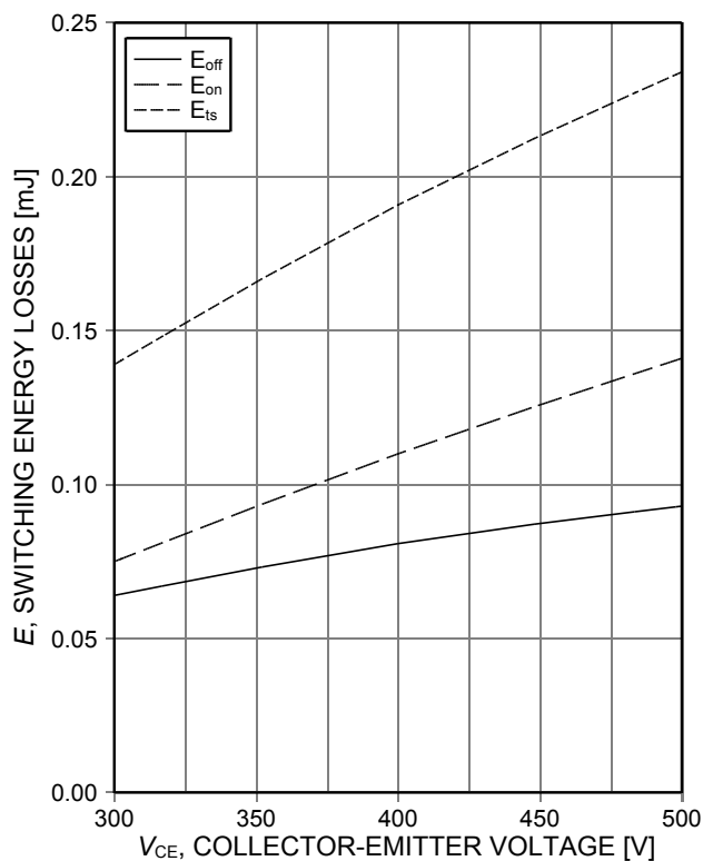
Figure 16. Typical switching energy losses as a function of collector emitter voltage (inductive load, T_{vj}=175^\circ\text{C} , V_{GE}=15/0\text{V} , I_C=4\text{A} , r_G=43\Omega , Dynamic test circuit in Figure E)
