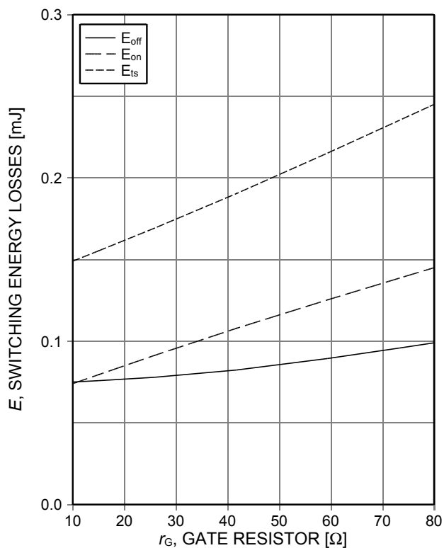
Figure 14. Typical switching energy losses as a function of gate resistor (inductive load, T_{vj}=175^\circ\text{C} , V_{CE}=400\text{V} , V_{GE}=15/0\text{V} , I_C=4\text{A} , Dynamic test circuit in Figure E)
