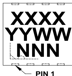
8-Lead DFN (3x3x0.9 mm)
