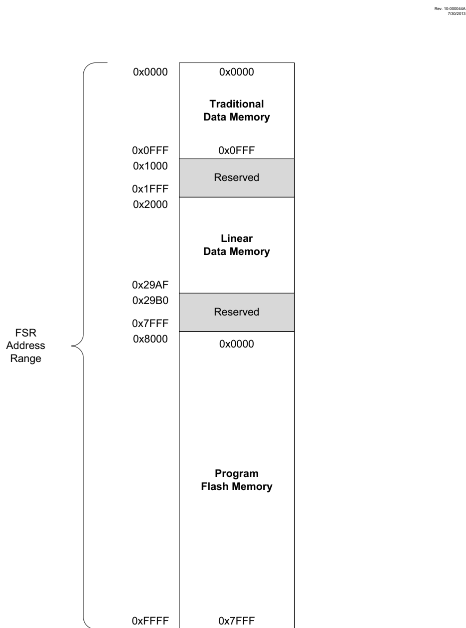
FIGURE 3-9: INDIRECT ADDRESSING
