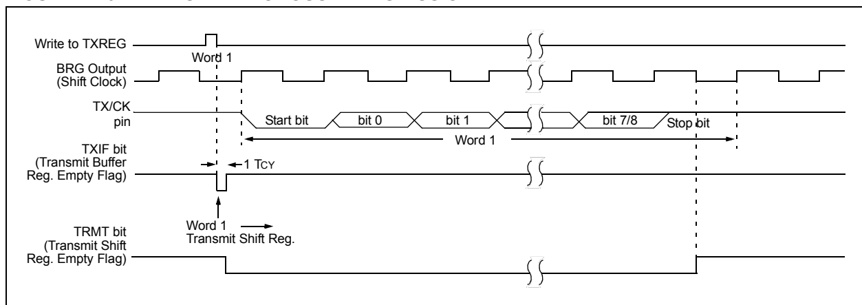
FIGURE 21-3: ASYNCHRONOUS TRANSMISSION
